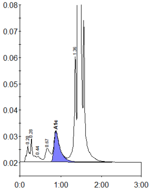
Peak table - ID: 10619523
